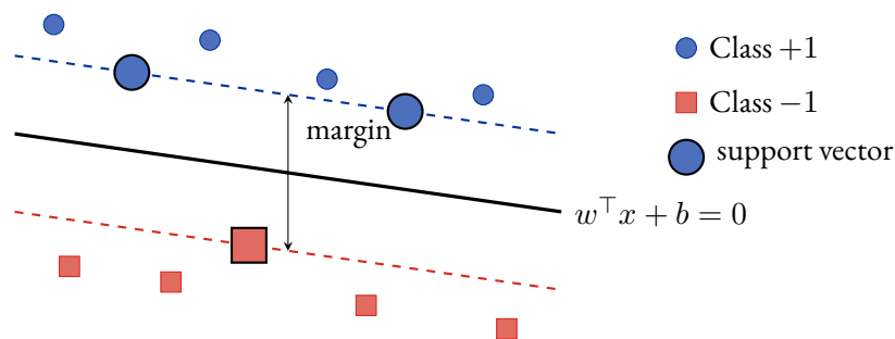
Figure 10.3: The maximum-margin hyperplane of a Support Vector Machine. The decision boundary w^\top x + b = 0 is placed to maximize the margin between the two classes; the support vectors (outlined) are the points that lie exactly on the margin boundary and alone determine the solution.
