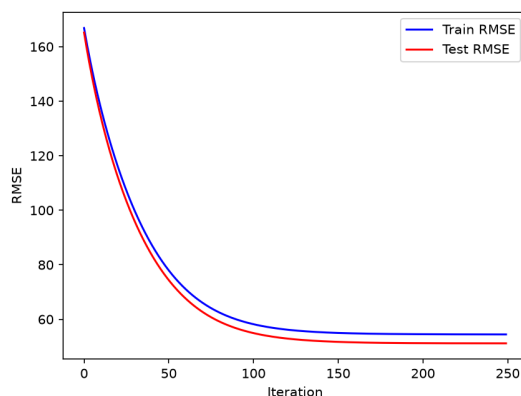
Figure 2.4: Learning curve: training and test RMSE of Lasso regression across gradient descent iterations.
